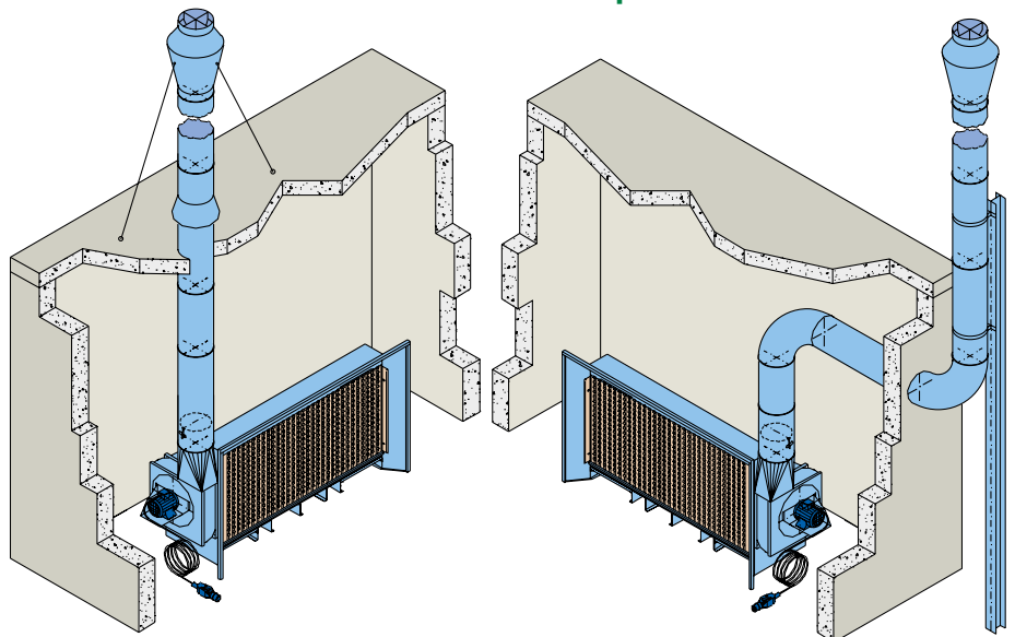
Schuko FarbMax with exhaust air ducting through the roof.
